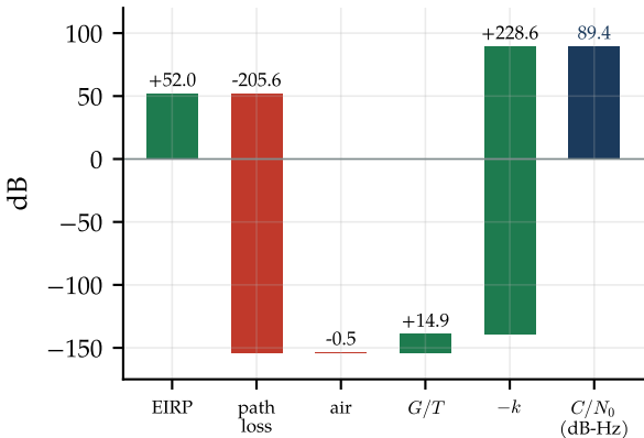
A Ku-band TV downlink in five terms
