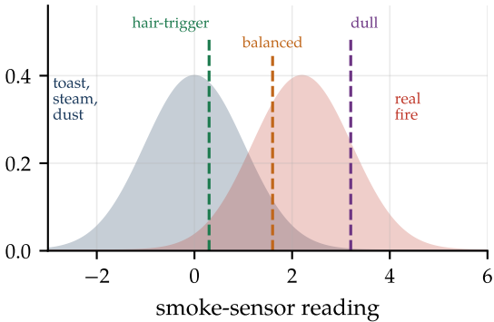
same sensor, three thresholds
