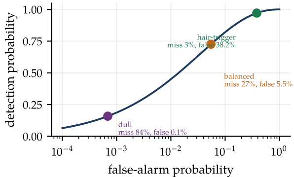
the ROC: one curve, every threshold
