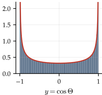
sine at random instants
