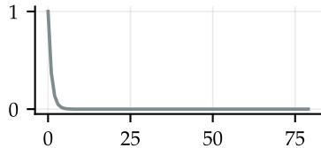
autocorrelation R(\tau)
