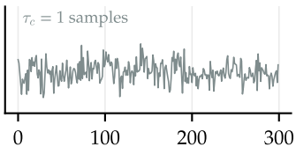
sample path
