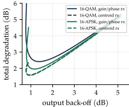
RRC 0.2, rate-3/4 threshold
