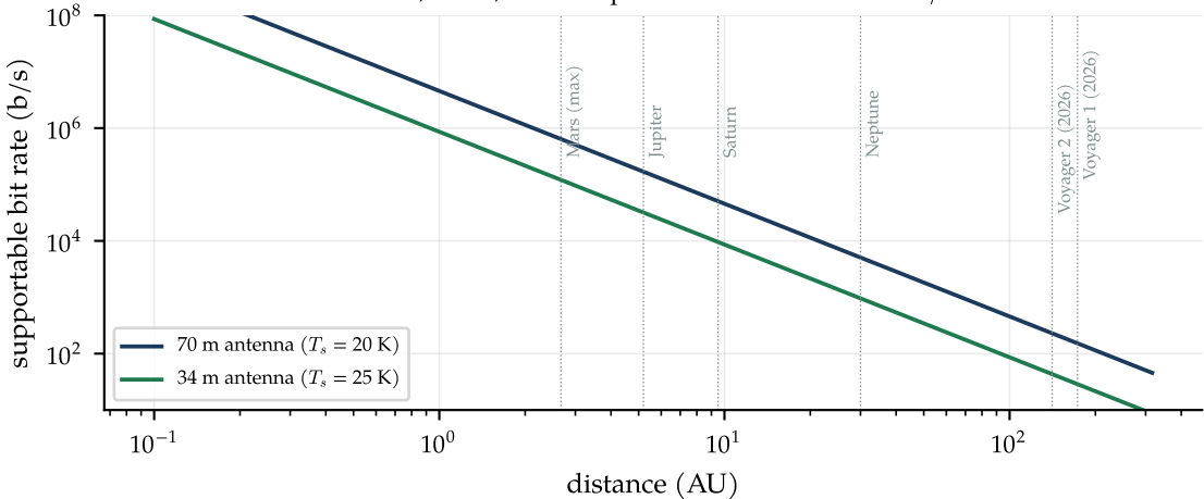
A 20 W, 3.7 m, X-band spacecraft link: rate falls as 1/d^2
