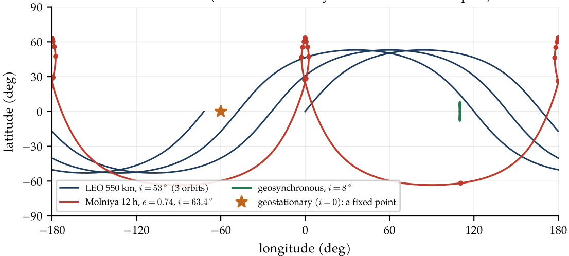
Ground tracks (dots on the Molniya track are one hour apart)
