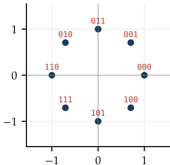
8-PSK (Gray)
