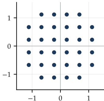
32-cross QAM
