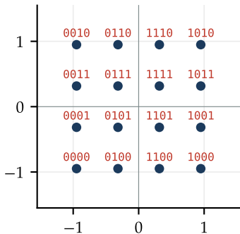
16-QAM (Gray)
