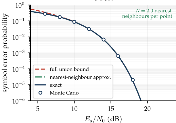
8-PSK
