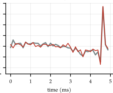
(c) sum: SNR 10.7 dB (17 bits for pulses)
