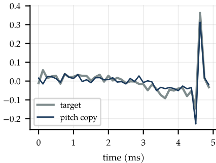
(a) adaptive codebook: lag 134 = 16.8 ms SNR 8.2 dB
