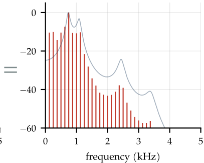
buzz \times tube = vowel /a/
