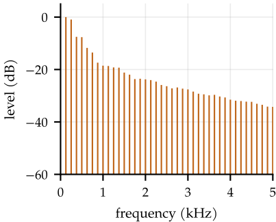
the buzz: harmonics of 125 Hz
