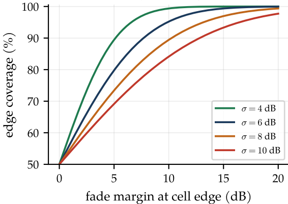
(a) probability of coverage at the edge
