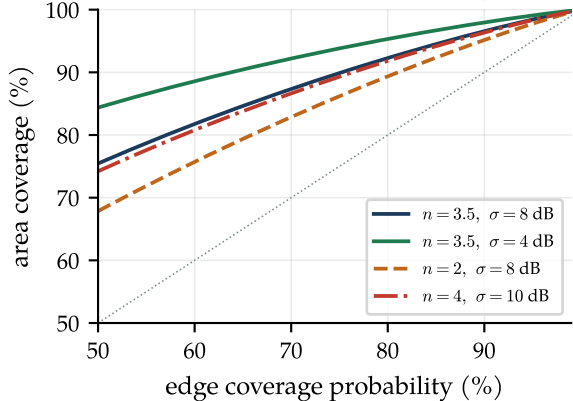
(b) Jakes--Reudink area coverage
