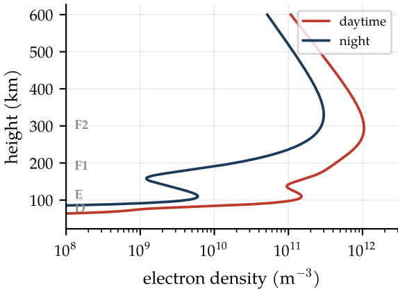
(a) ionospheric layers (illustrative)
