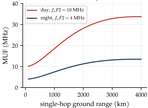
(b) \text{MUF} = f_o \sec \theta_i , layer at 300 km
