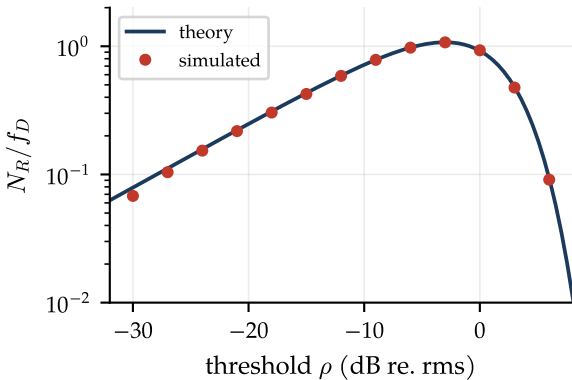
(a) level-crossing rate
