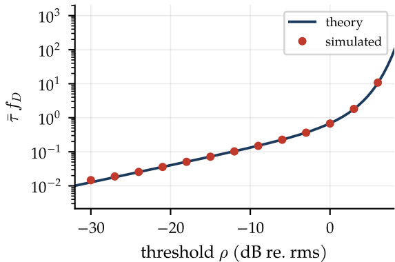
(b) average fade duration
