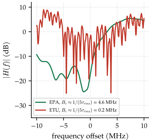
(b) one realisation over 20 MHz
