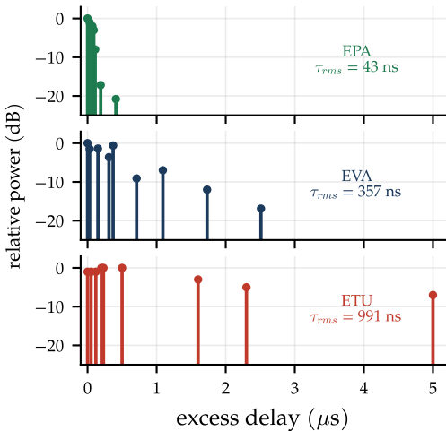
(a) LTE power delay profiles (dB)
