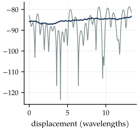
(b) zoom: 2 m around 400 m
