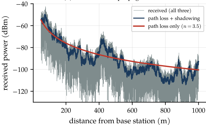
(a) three scales of propagation, 2 GHz
