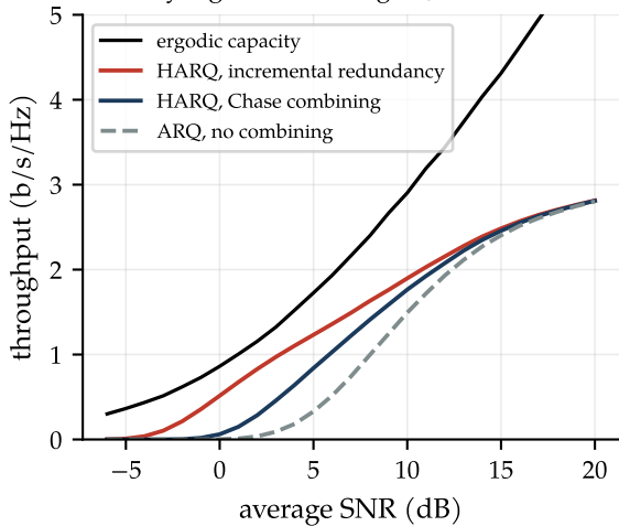
Rayleigh block fading, R_0 = 3 , \leq 4 tx
