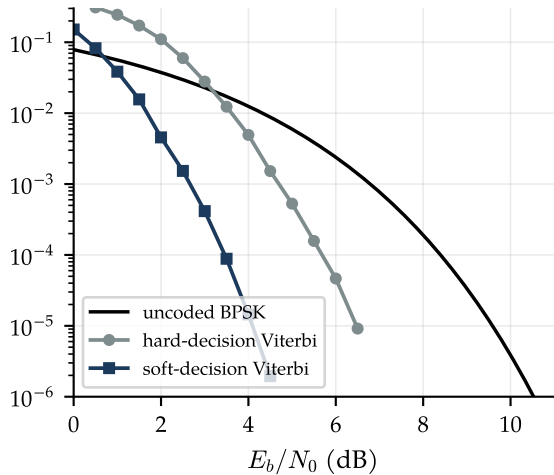
Convolutional K = 7, R = 1/2
