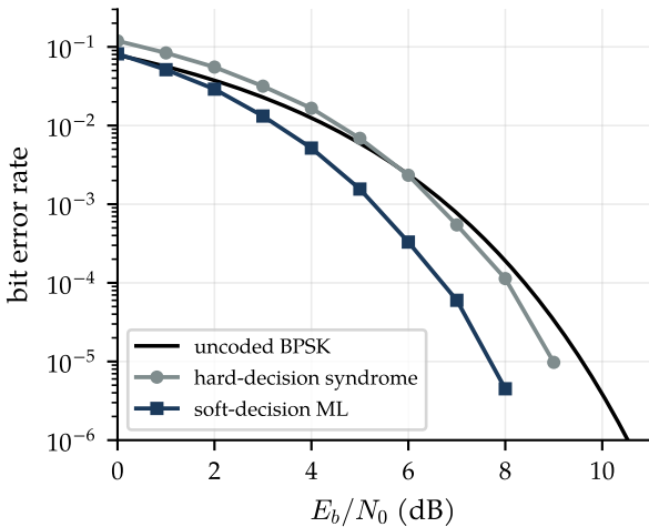
Hamming (7,4)
