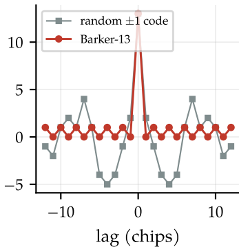
Autocorrelation R_x(\tau)
