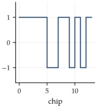
Barker-13 code
