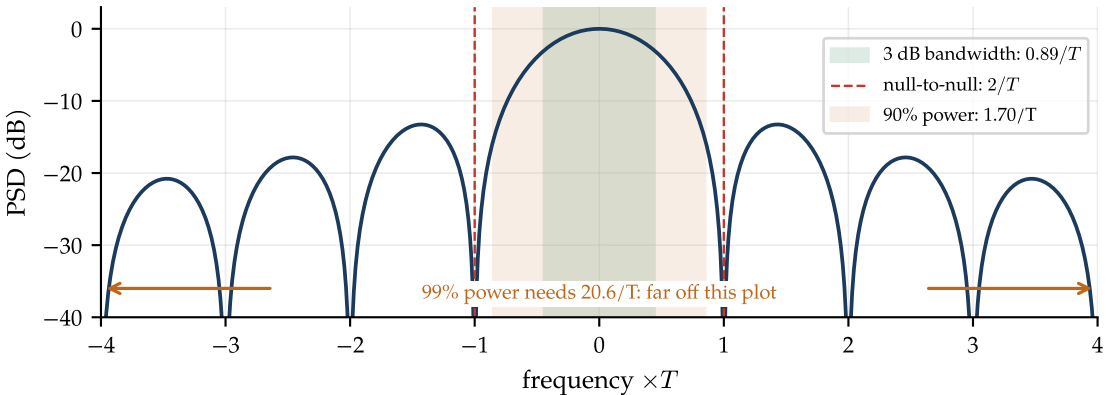
Bandwidth of a rectangular pulse of duration T depends on the definition
