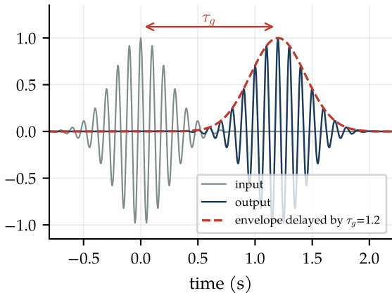
Envelope moves by \tau_g , carrier phase by \tau_p (0.3 s)
