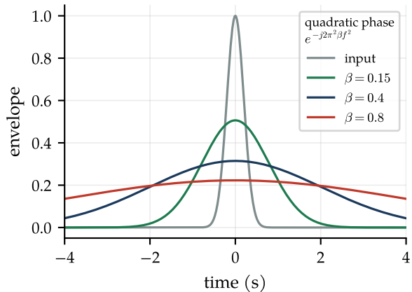
Dispersion: linear group delay spreads a pulse
