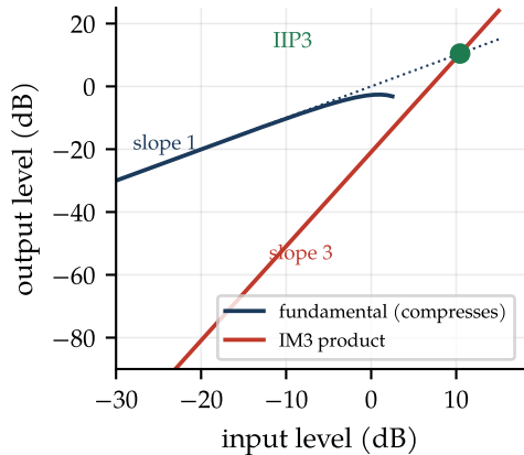
Third-order intercept
