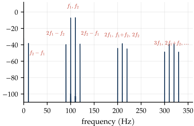
Two tones through y = a_1x + a_2x^2 + a_3x^3
