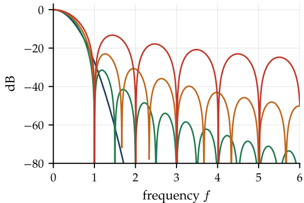
Their spectra (Gaussian lowest)
