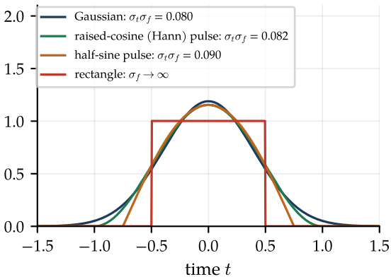
Four unit-energy pulses
