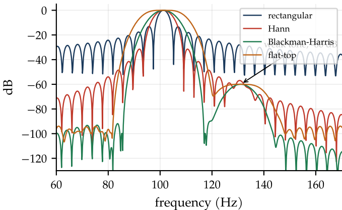
Leakage: a -60 dB tone 30 Hz away
