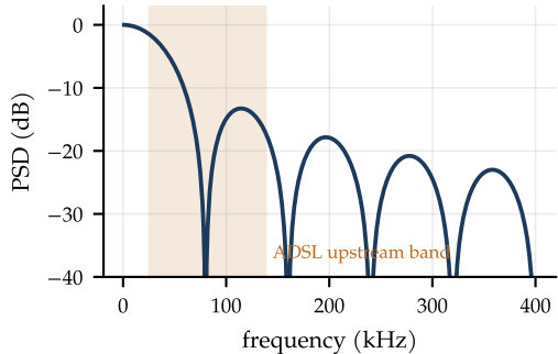
ISDN's spectrum: first null at 80 kHz
