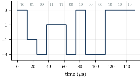
2B1Q: two bits per quaternary symbol, 80 kBd
