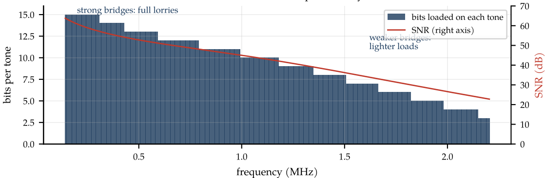
ADSL2+ on 2 km of 0.4 mm cable: 4471 bits per DMT symbol, about 18 Mb/s
