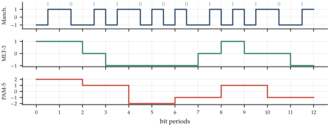
the same twelve bits: 10BASE-T, 100BASE-TX and (one pair of) 1000BASE-T
