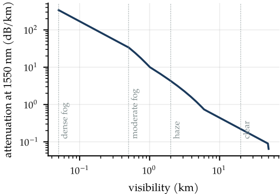
free-space optics vs the weather (Kim model)
