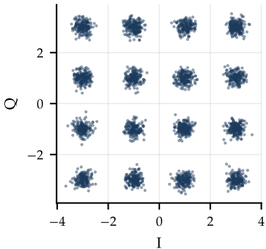
coherent receiver: field (16 points)
