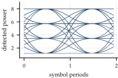
back to back
