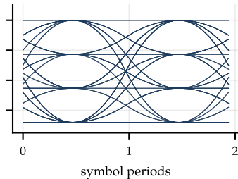
2 km, O band ( D \approx 0 )
