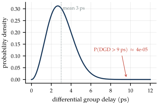
PMD: Maxwellian DGD, 1000 km of modern fibre
