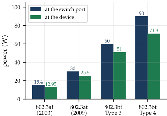
Power over Ethernet classes
