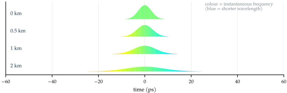
a 4 ps pulse at 1550 nm in standard fibre: the blue runners pull ahead
