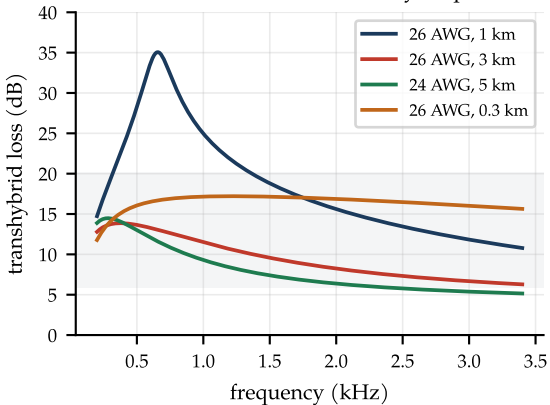
one balance network, many loops
