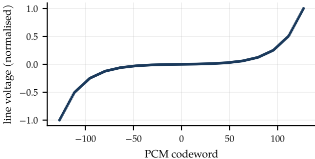
the 255 \mu -law levels a line card can produce
