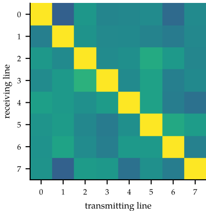
without vectoring
