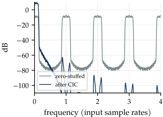
CIC interpolator, R = 8 , N = 4
