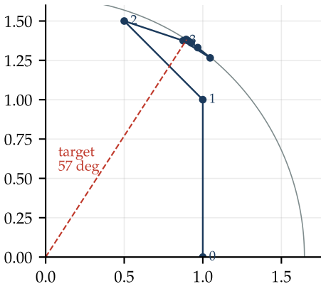
rotation-mode trajectory (radius grows to 1/K \approx 1.647 )
