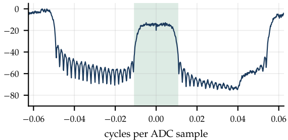
2. NCO to 0 Hz, CIC \downarrow 8
