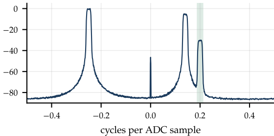
1. ADC capture (wanted at +0.2)
