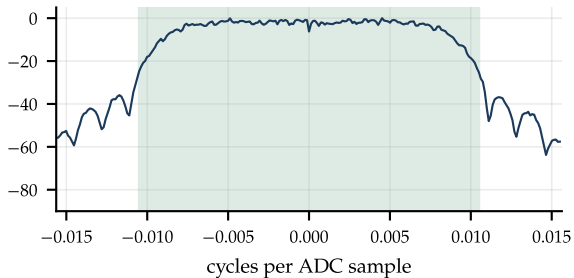
4. channel FIR \downarrow 2 : done
