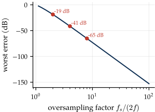
cubic Farrow interpolator error
