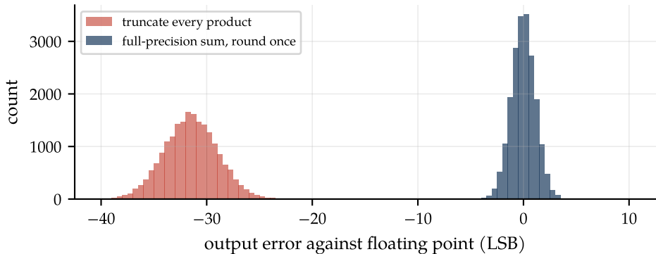
bit-true simulation of a 63-tap, 16-bit FIR
