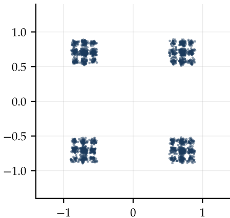
6th-order elliptic: EVM -17 dB
