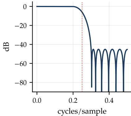
magnitude: symmetric about f_s/4
