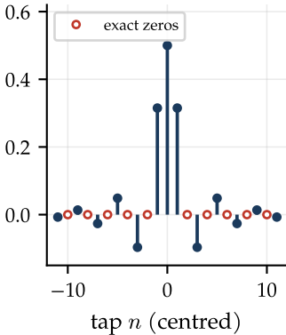
23-tap half-band h[n]
