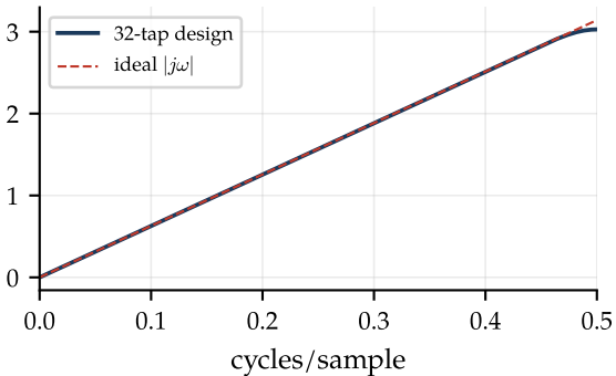
differentiator (type IV)
