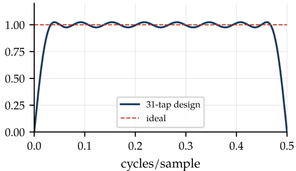
Hilbert transformer (type III)
