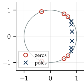
elliptic pole-zero
