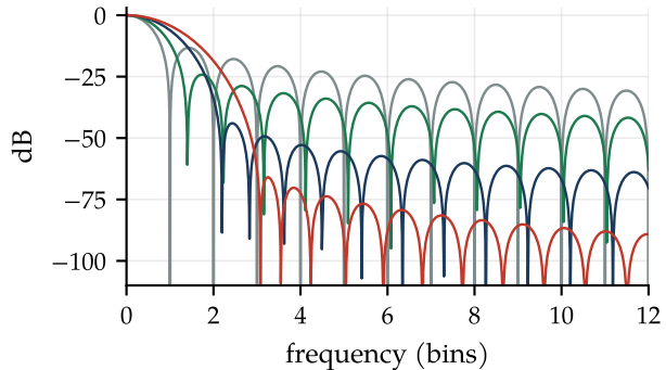
spectra: wider lobe, lower sidelobes
