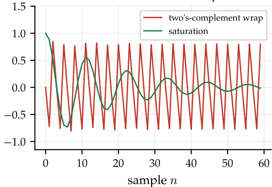
overflow oscillation, zero input
