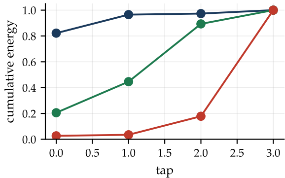
energy arrives earliest for minimum phase
