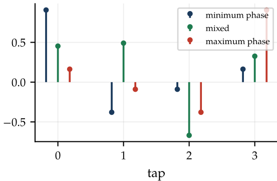
three filters with identical |H|
