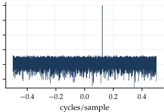
10-bit phase, with dither: worst spur -84 dBc
