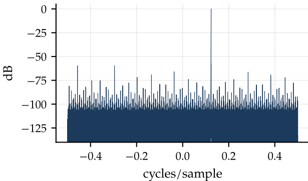
10-bit phase, truncated: worst spur -60 dBc
