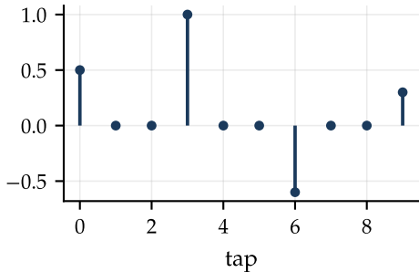
H(z^3) : taps 3 samples apart
